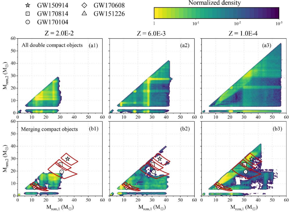
Fig. 1. Mass of the less massive remnant ( M_{\text{rem}, 2} ) as a function of the mass of the more massive remnant ( M_{\text{rem}, 1} ) in all compact-object binaries (top row), and in the compact-object binaries merging within a Hubble time (bottom row). The logarithmic colour bar represents the number of remnants per cell, normalized to the maximum cell-value of each plot. Each cell is a square with a side of 0.5 M . Left-hand column (labelled as 1): Z = 2 \times 10^{-2} ; central column (2): Z = 6 \times 10^{-3} ; right hand column (3): Z = 10^{-4} . The open symbols are the BH mergers detected by LIGO/Virgo in O1 plus the first results of O2. The solid red lines around the open symbols define the 90% credible interval on the chirp mass and the mass ratio of each GW event.
